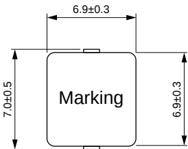
Dimensions: [mm]
