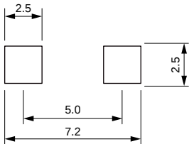
Land Pattern: [mm]
