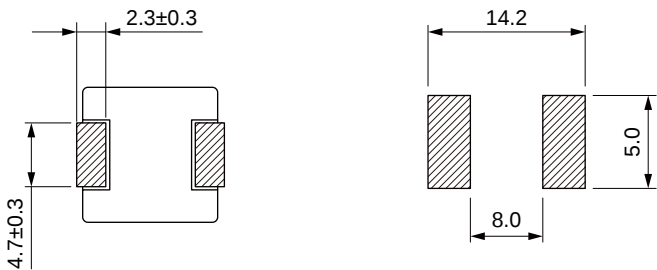
Land Pattern: [mm]
